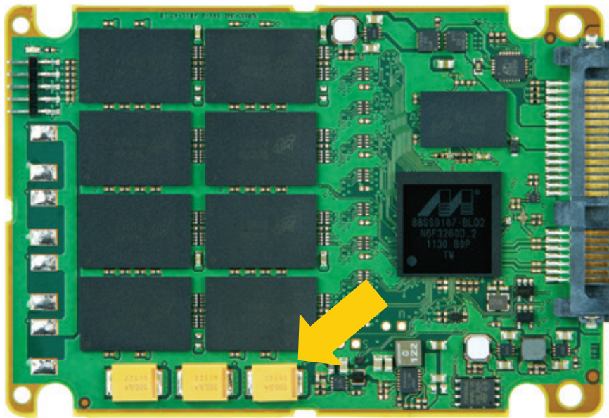
Figure 4: Tantalum Hold-Up Capacitors on Micron's P400m Enterprise SSD
