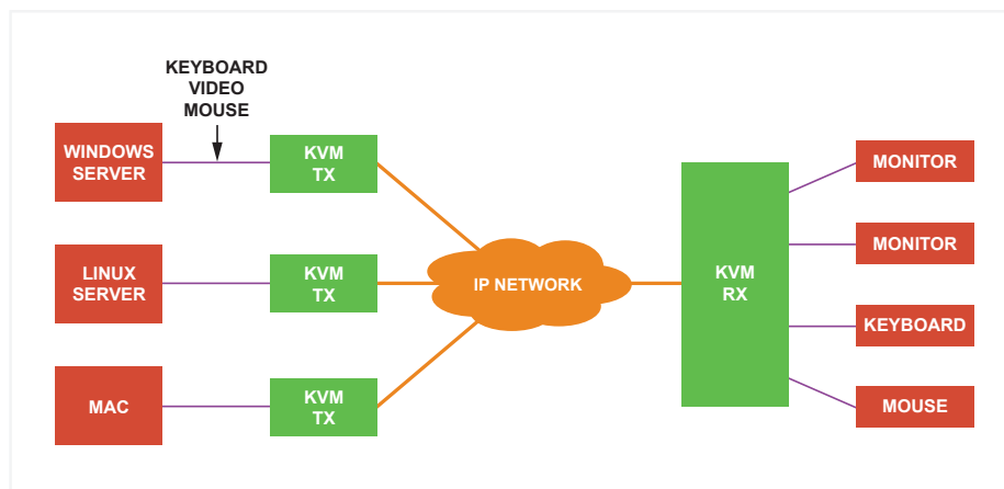
Figure 1 – KVM transmitters and receivers are used to multiplex the video and audio streams, keyboard and mouse signals onto IP networks so they can be decoded at the user's desk. As well as improving security, this method also provides a much-enhanced working environment..
